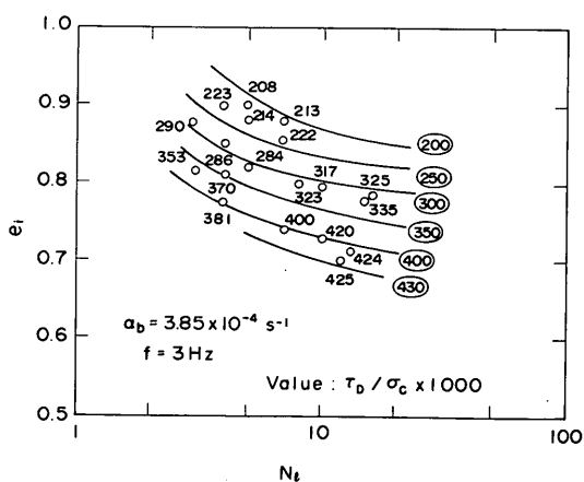
圖-9.11 f e_i \sim N_i \sim \tau_D / \sigma_c 關係 ( \alpha_b = 3.85 \times 10^{-4} \text{ s}^{-1} , f = 3 \text{ Hz} )
