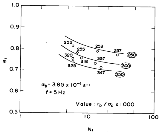
圖-9.11 d e_i \sim N_i \sim \tau_D / \sigma_c 關係 ( \alpha_b = 3.85 \times 10^{-4} \text{ s}^{-1} , f = 5 \text{ Hz} )
