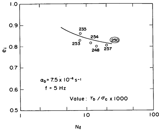
図一9.11g e_i \sim N_i \sim \tau_D/\sigma_c 関係 ( \alpha_b = 7.5 \times 10^{-4} \text{ s}^{-1} , f = 5 \text{ Hz} )
