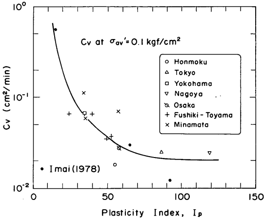
図-6.23a 圧密係数と塑性指数の関係 ( \sigma_{av}' = 0.1 \text{ kgf/cm}^2 )
